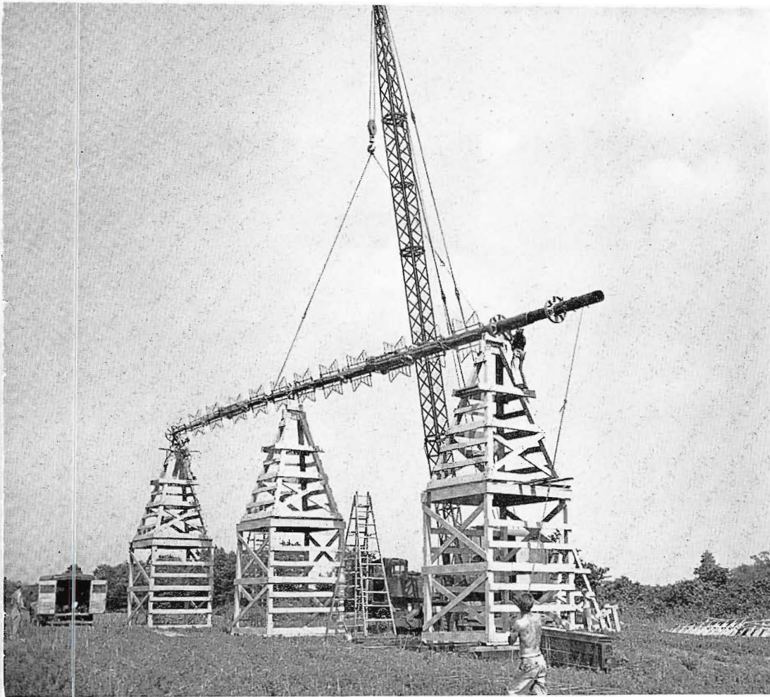
FIG. 8. Antennas were placed on 25-foot high supports and then rotated to insure that radiating patterns are not affected by proximity of ground.
