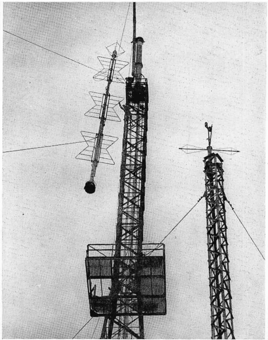
FIG. 4. The RCA TT-3B Superturnstile Antenna nearing the top of the tower. The temporary antenna can be seen at the right, foreground.
