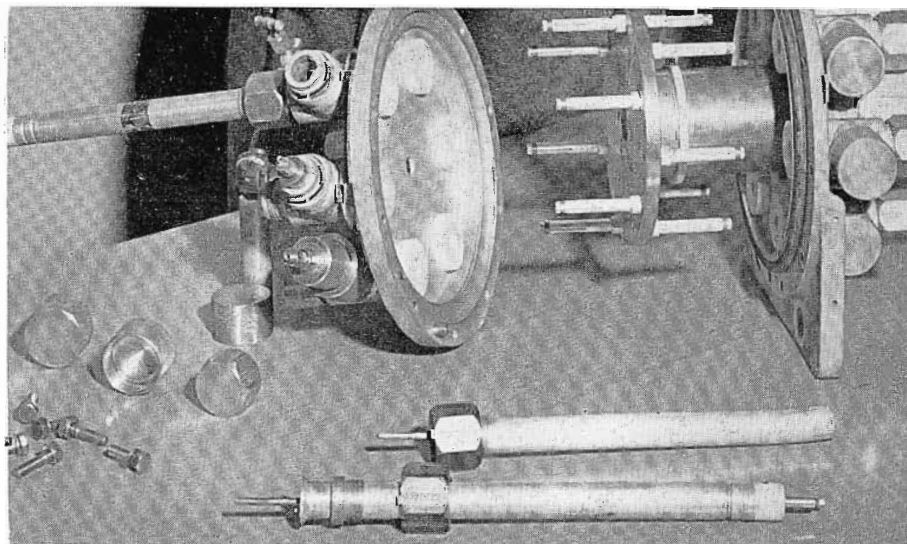
FIG. 3. A junction box of advanced design is employed in the 12-section antennas. Reflectometer wells enable a constant indication of electrical condition of feedlines.
