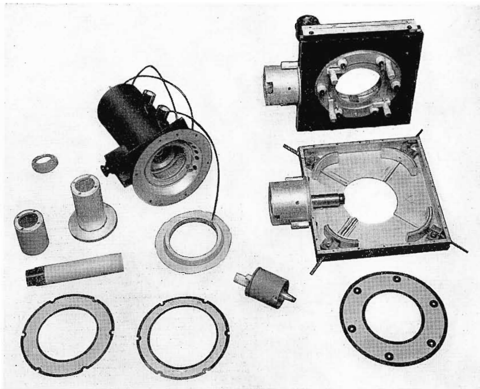
FIG. 11. PA cavity completely disassembled.
