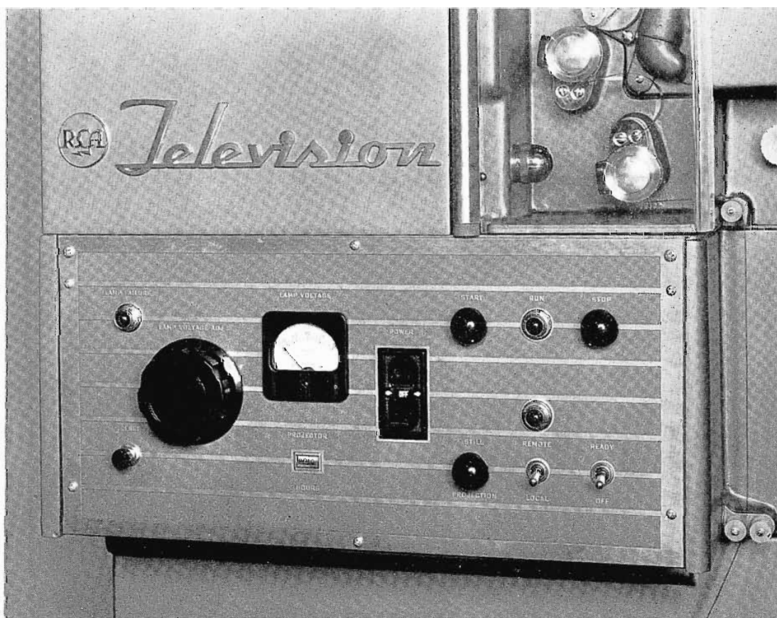
FIG. 14. Closeup of TP-6A control panel which is conveniently located for the operator.
