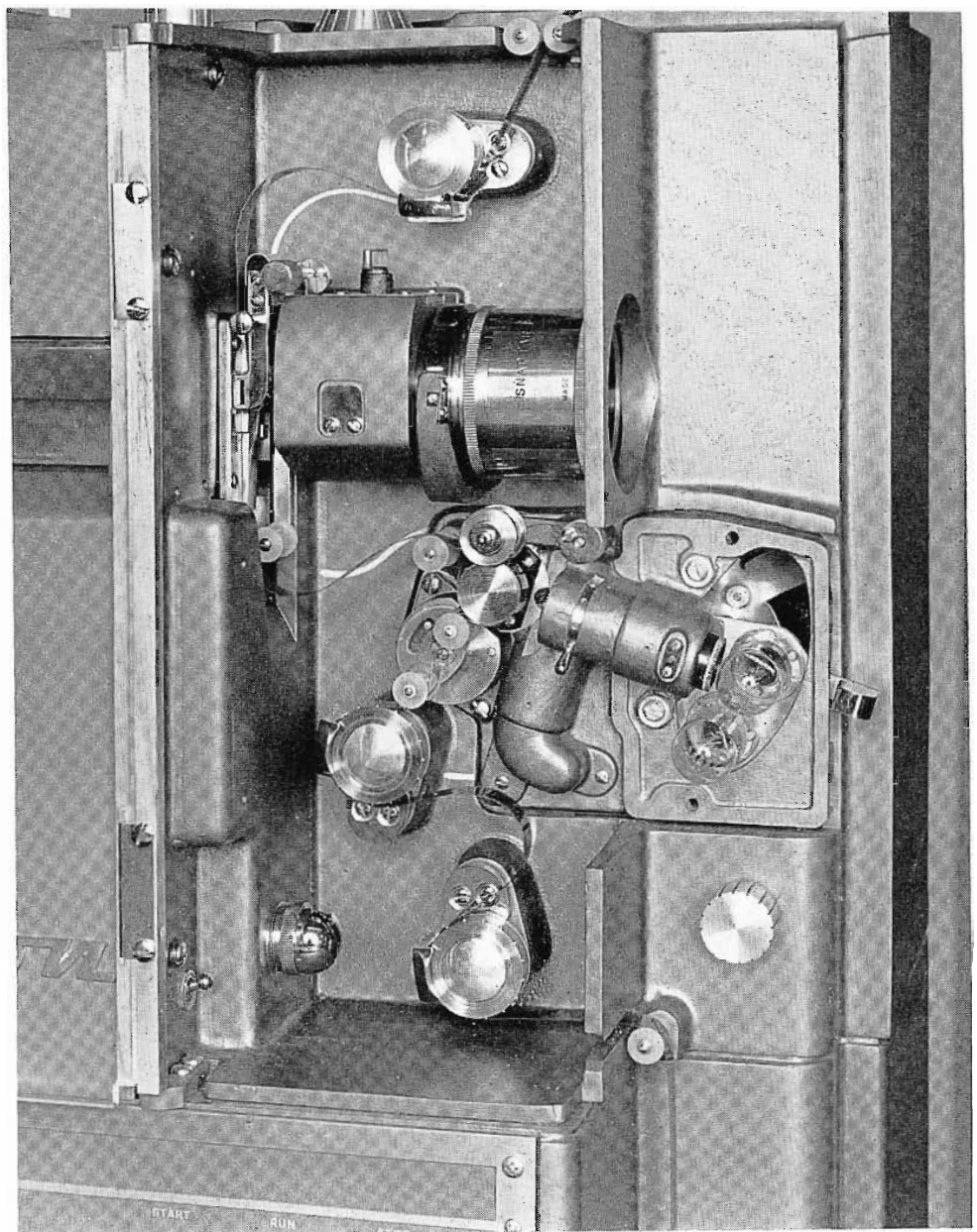
FIG. 7. View of the TP-6A Projector showing the optical components, film path and focus controls.
