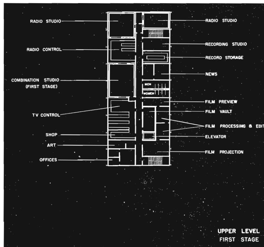
FIG. 9. Upper level plan, during first stage.
