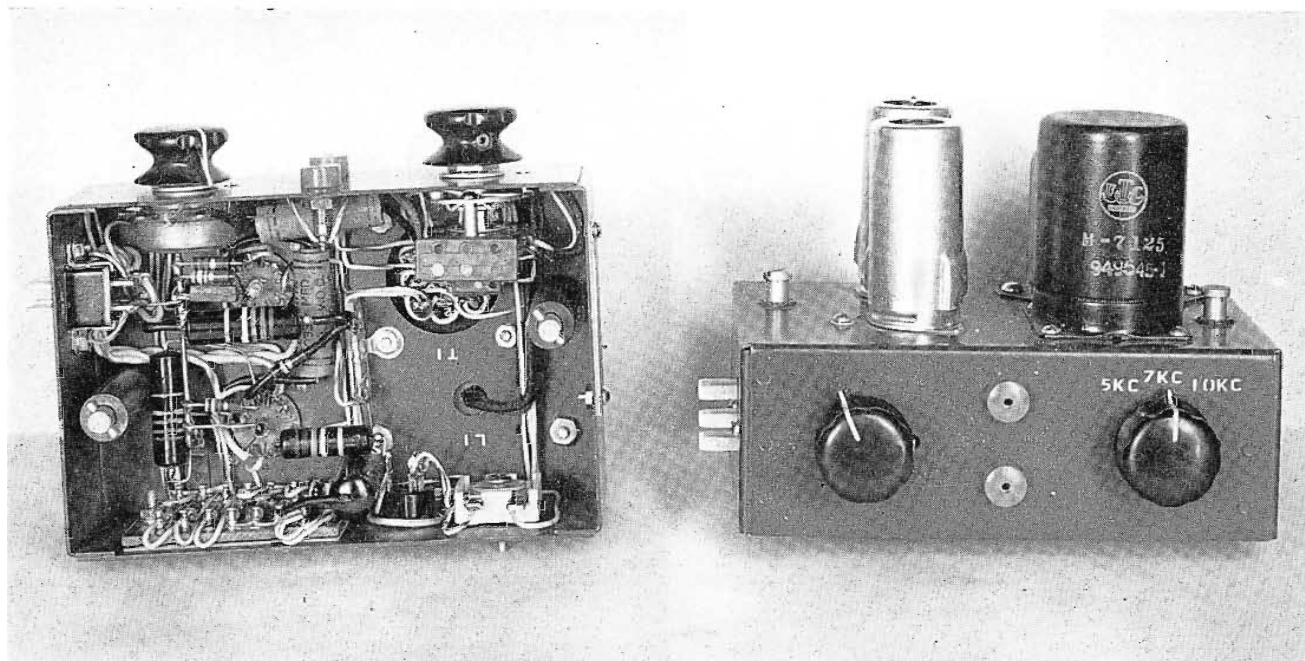
FIG. 12. Under-chassis view and front view of preamplifier chassis.
