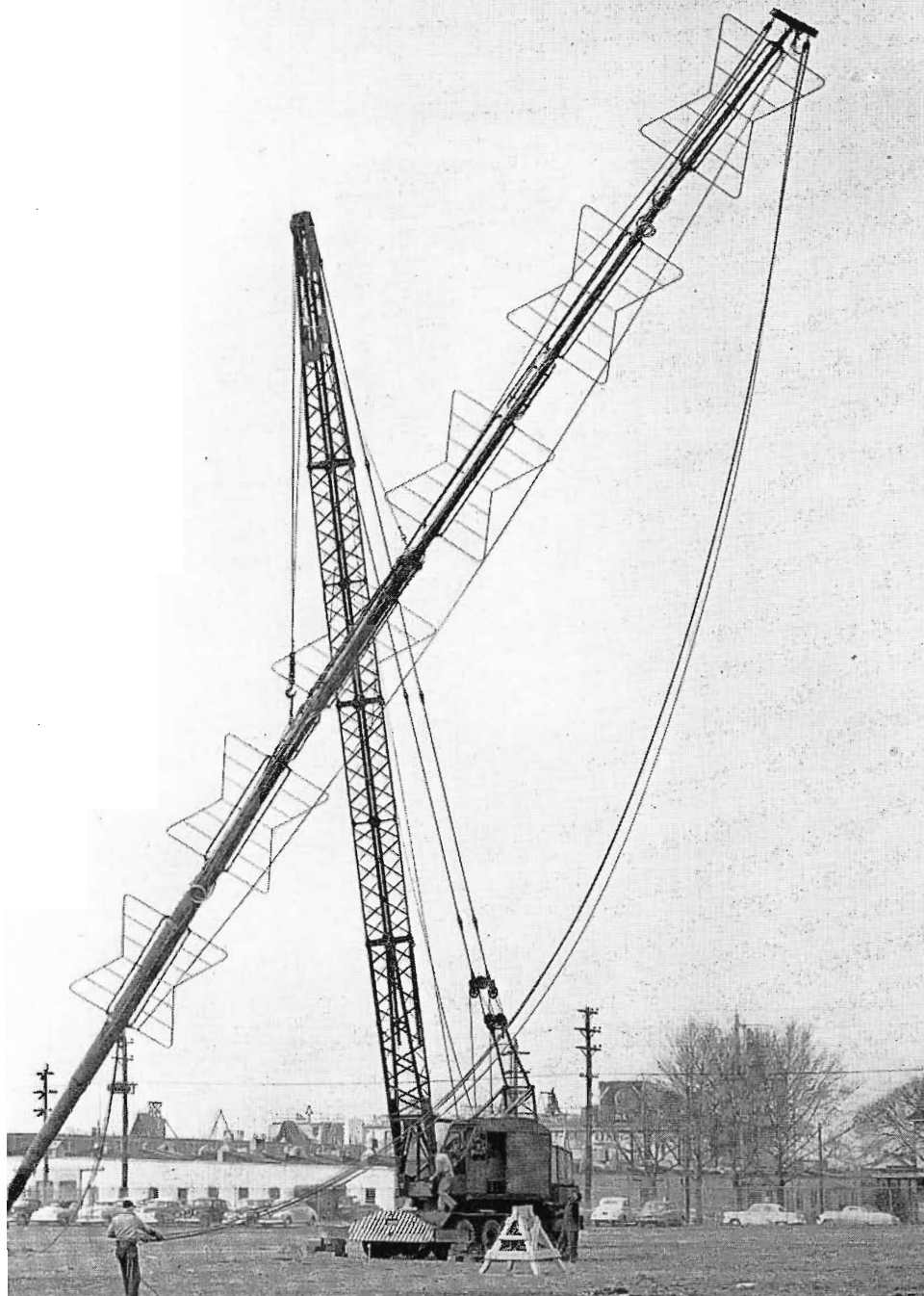
FIG. 7. The TF-6AL Superturnstile being raised to vertical position so that a "double check" can be made of the measurements obtained when horizontally positioned.
