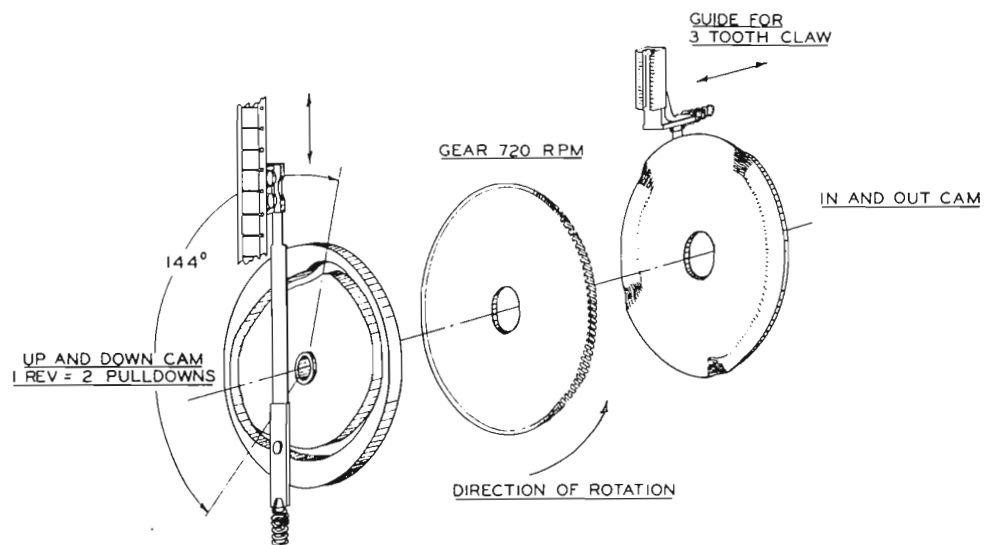
Fig. 9. Diagram showing an exploded view of the TP-6A intermittent.
