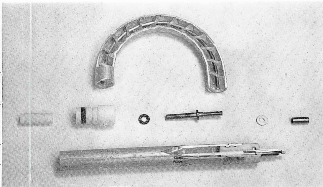
FIG. 2. Exploded view of a section of Styroflex feedline with segments cut out to illustrate construction.
