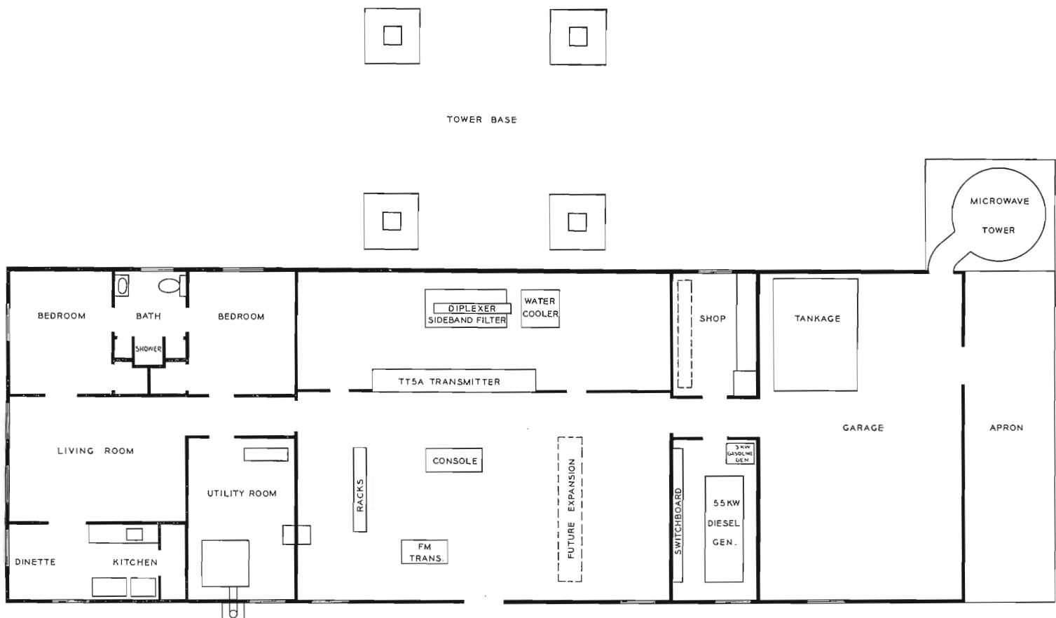
FIG. 6. Floor plan of the KDYL-TV transmitter building on Mt. Vision. The antenna tower is located as near transmitter as possible in order to keep the transmission line short. Note also that inside access to the microwave tower is provided.
