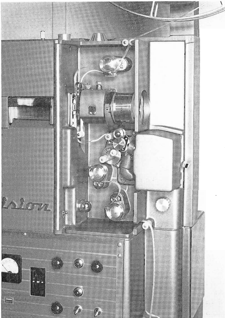
FIG. 10. Closeup view of the TP-6A sound reproduction assembly.
