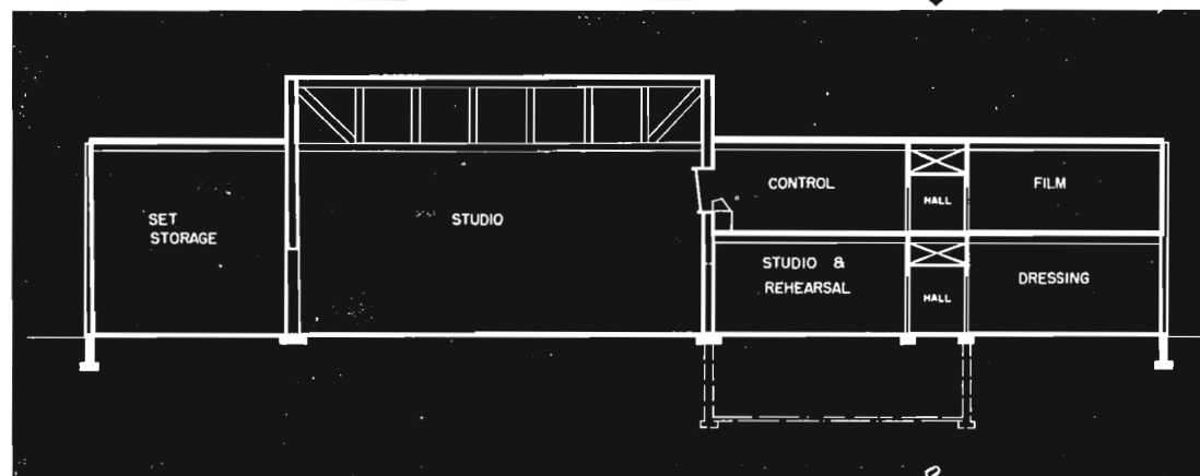
FIG. 5. Cross-sectional drawing which shows vertical relationships among various sections of building.
