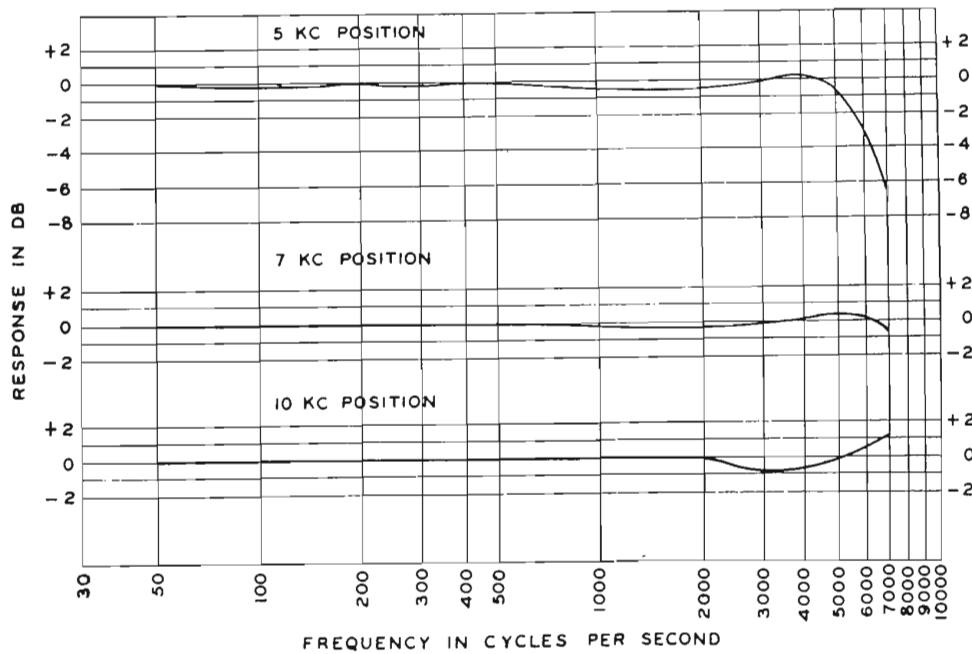
FIG. 13. Overall response curves of a typical TP-6A Projector using "SMPTE" multifrequency test film.
