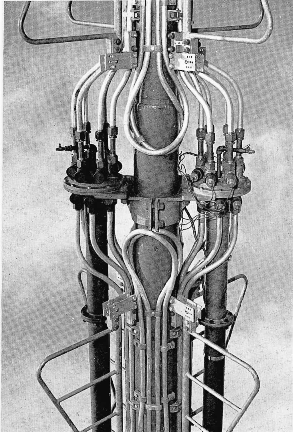
FIG. 4. Closeup view of new junction box as it appears installed on a 12-section antenna (TF-12AH). Test reflectometers are in use in the right hand junction box.
