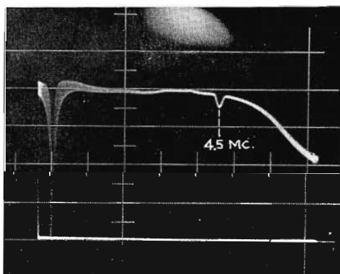
FIG. 14. Overall frequency response of the TTU-1B—Marker at 4.5 mc.
