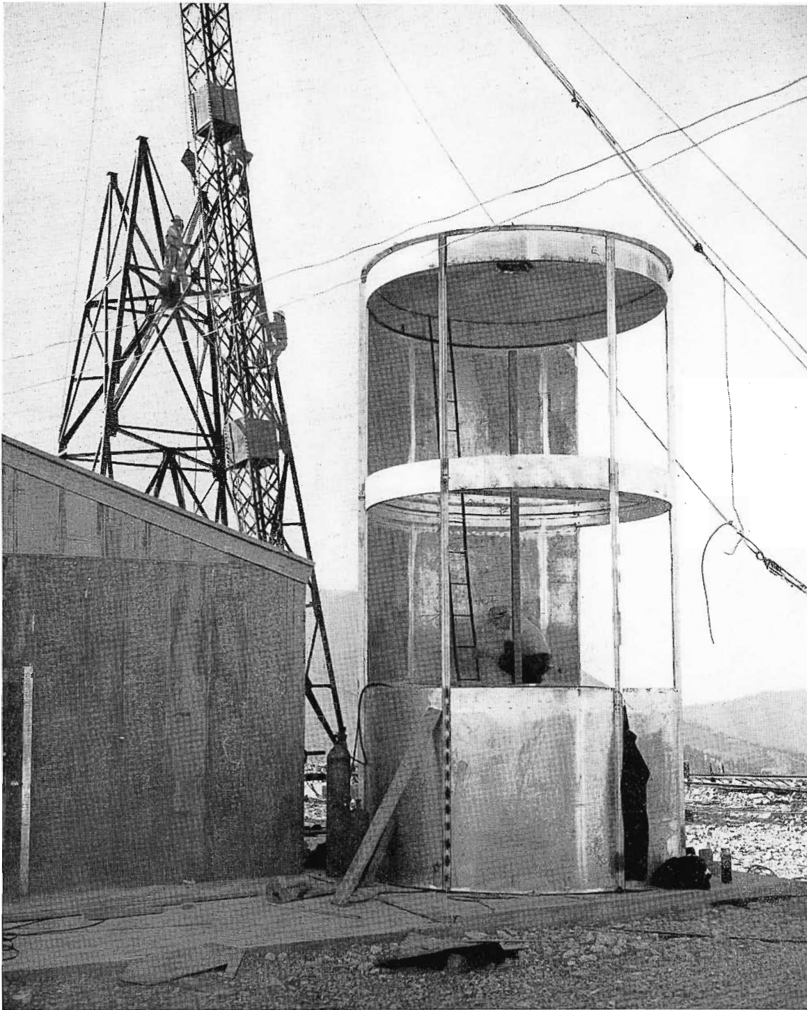
FIG. 9 (left). A unique feature of the KDYL-TV installation is a microwave "tower", shown here during construction. Two station-owned RCA microwave links provide video circuits from the studios in Salt Lake City. The receiving parabolas are mounted at two levels, as shown in the diagram on the opposite page. The enclosure protects them from the weather and makes maintenance easy.
