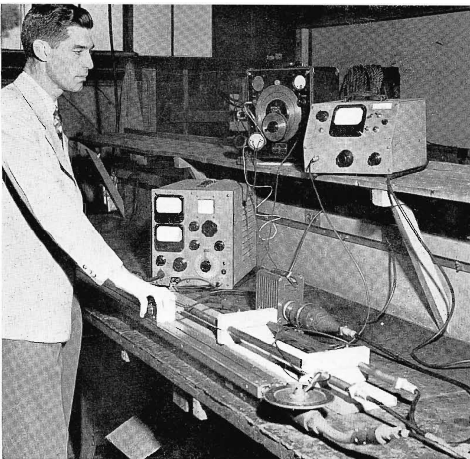
FIG. 5. Laboratory tests being conducted during development of the new feedlines and junction box.
