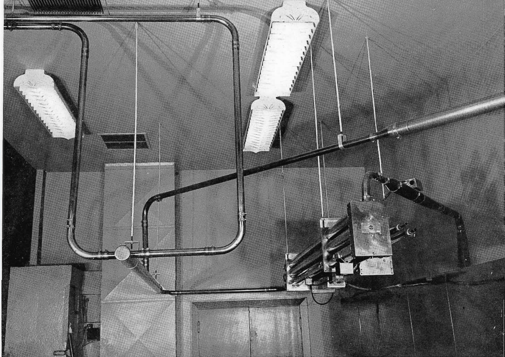
FIG. 6. Rear of transmitter showing diplexer, sideband filter, WM-20A Demodulator and inside transmission line. The line passes through the building wall just to the left of the picture. Gassing takes place just prior to leaving the building. One line is 90° longer than the other from the output of the diplexer to the upper left corner of the picture.
