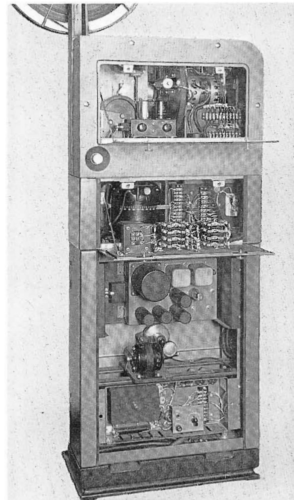
FIG. 11. Rear view of TP-6A with panels removed to show rack type assembly of power chassis and preamplifier.
