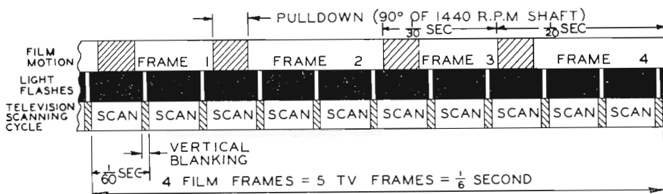
FIG. 6. Sketch showing time cycle comparison of TP-6A Professional Projector with that of the TP-16 Projector.
