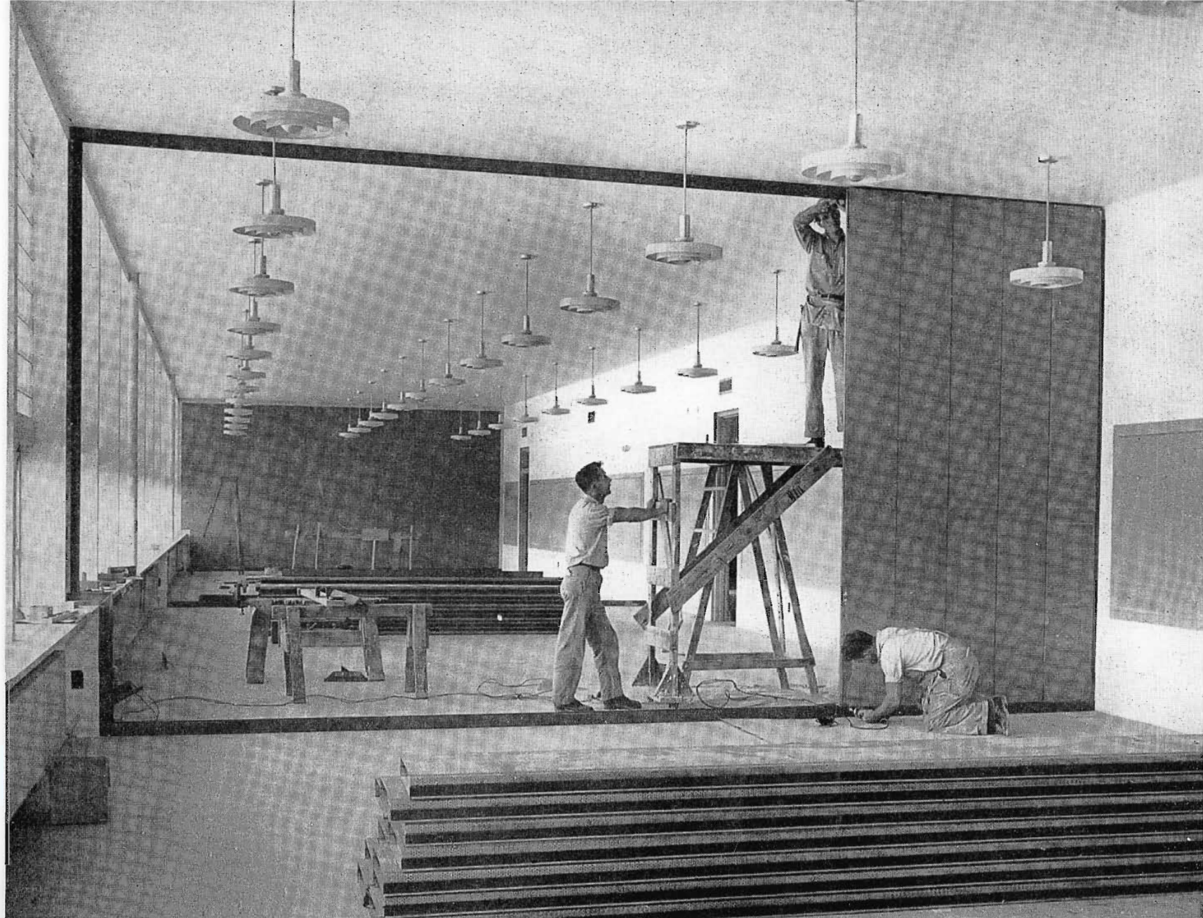
FIG. 10. Erecting removable steel panel as an interior partition.
