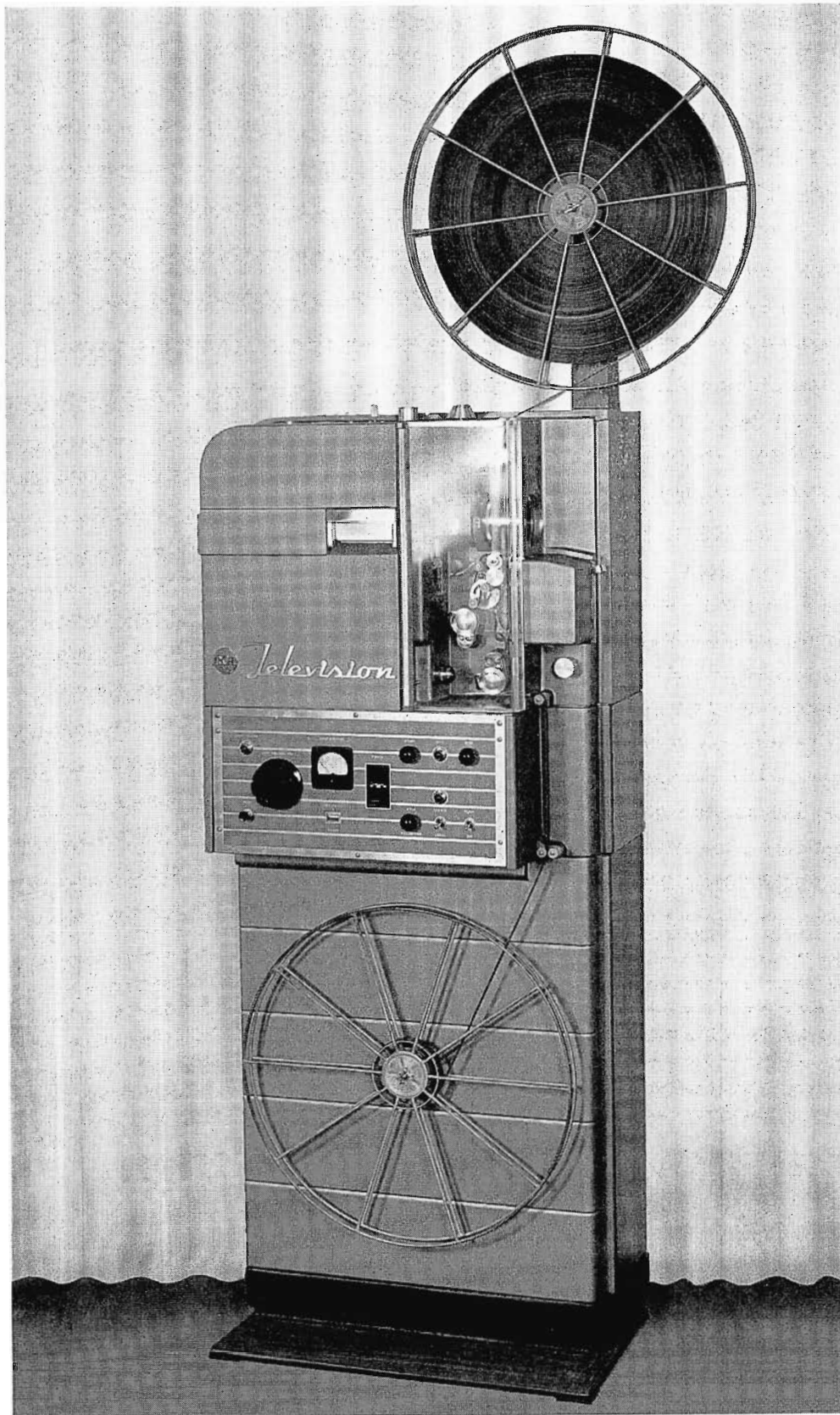
FIG. 1. The new RCA Professional Projector (TP-6A) which provides advanced operational and electrical features plus 4000-foot reels for uninterrupted programming.
