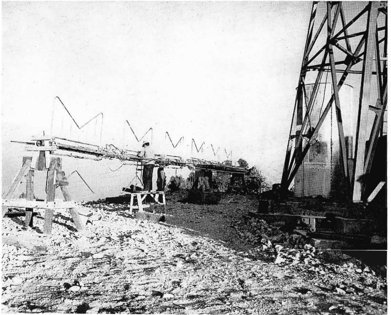
FIG. 2. Assembling the RCA six-bay turnstile at the KDYL-TV site. The base of the specially-built extra-heavy 100-foot tower on which the antenna is mounted is at the right. The microwave receiving antennas are enclosed in the silo-like structure behind the tower. Everything used at this very exposed site had to be of very heavy construction. The fact that the standard RCA turnstile antenna stands up under such extreme conditions is an indication of its high reliability.
