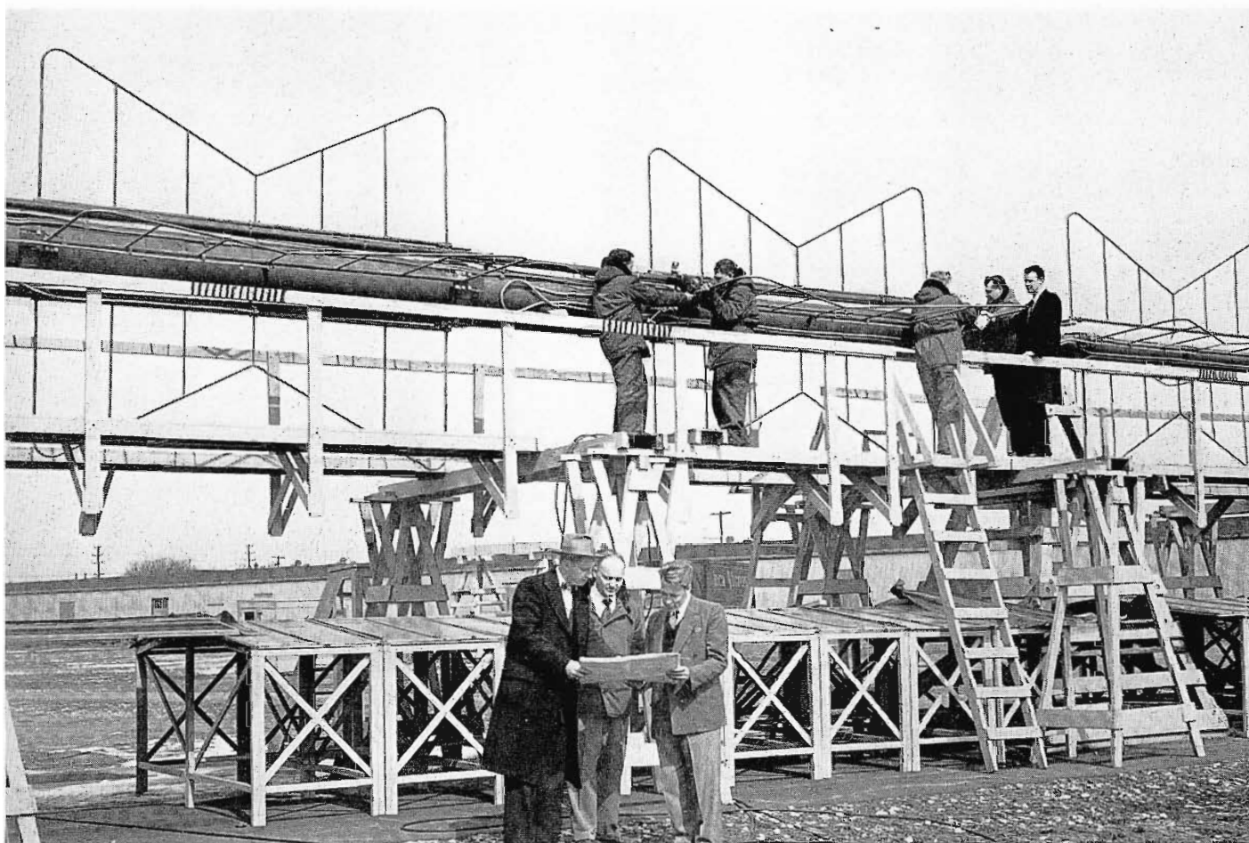
FIG. 6. Pilot model of the Type TF-6AL Superturnstile Antenna during field tests. Note space cloth framework below the antenna.
