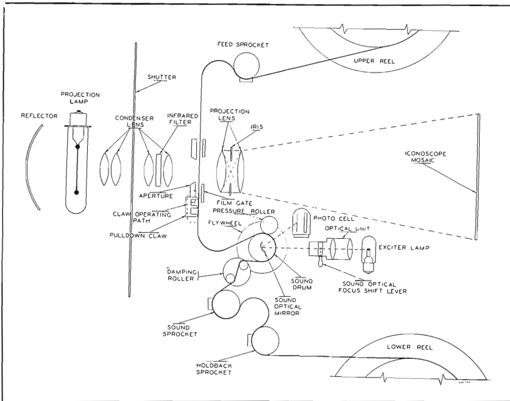
FIG. 4. Functional diagram of the TP-6A 16mm Projector showing optical component arrangement.
