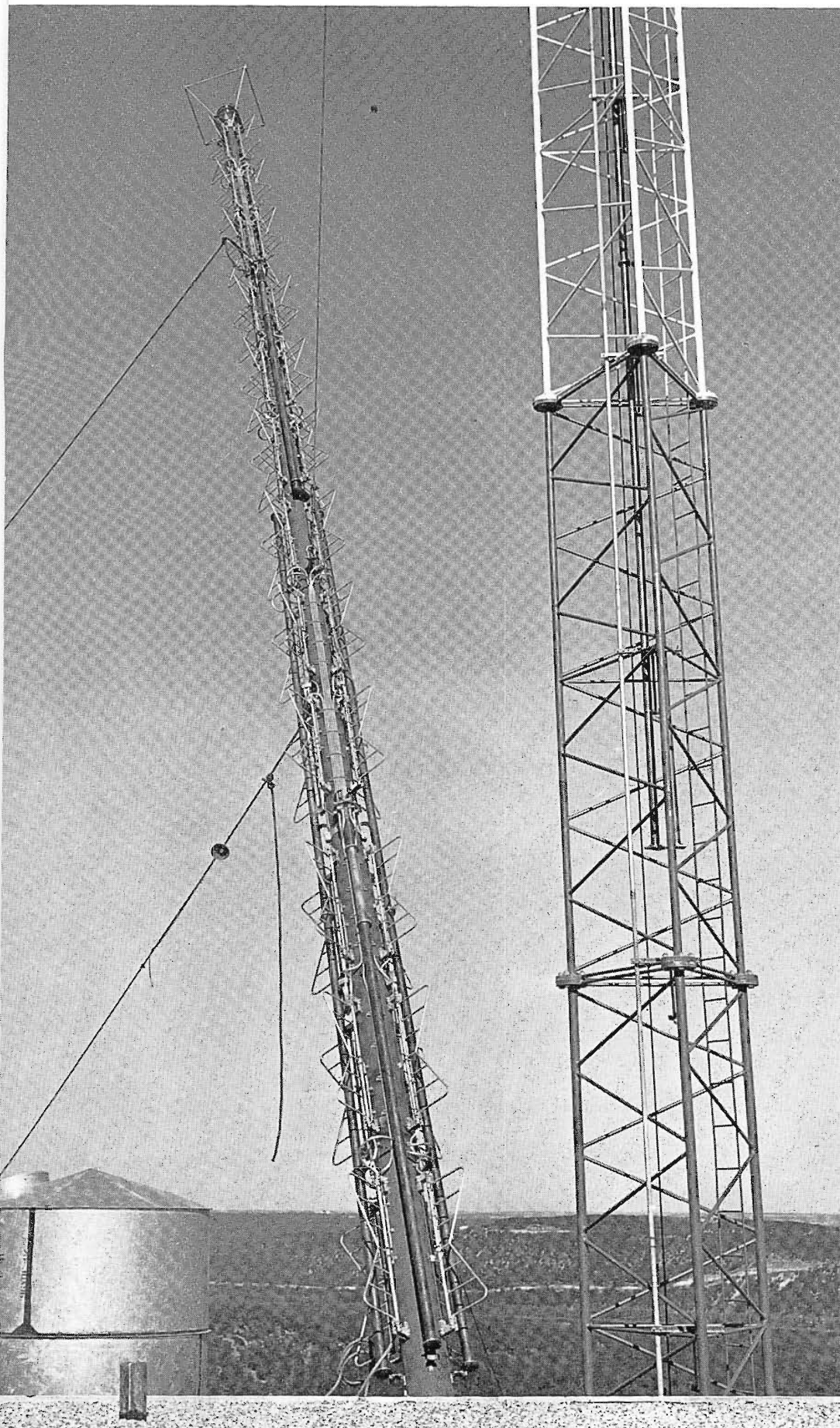
FIG. 1. Photo of the new 12-section (50-KW) antenna shown during installation at KTBC-TV, Austin, Texas.
