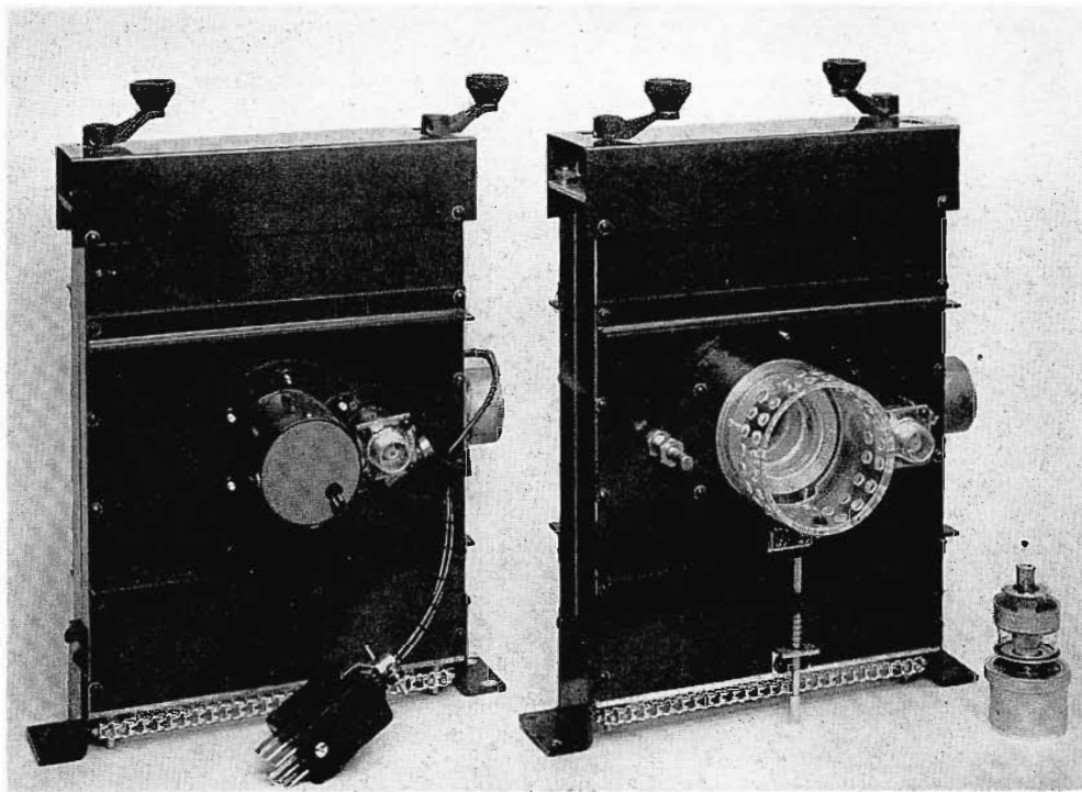
FIG. 8. Rectangular cavity for 6161 grounded grid doubler or amplifier.
