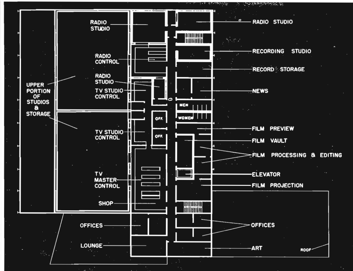
FIG. 4. Upper level plan of fully-expanded scheme.
