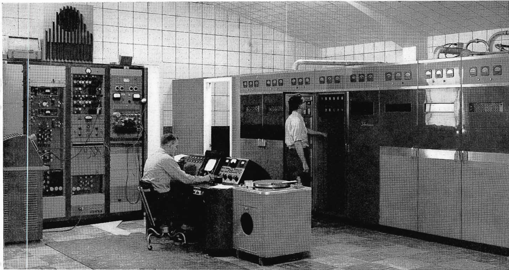
FIG. 8. The transmitter room on Mt. Vision. The RCA TT-5A Transmitter (right) works perfectly despite the rarefied atmosphere. Racks at the left contain video amplifiers, microwave relay receivers and monitoring units. With exception of a few minor units all equipment at KDYL-TV was supplied by RCA.
