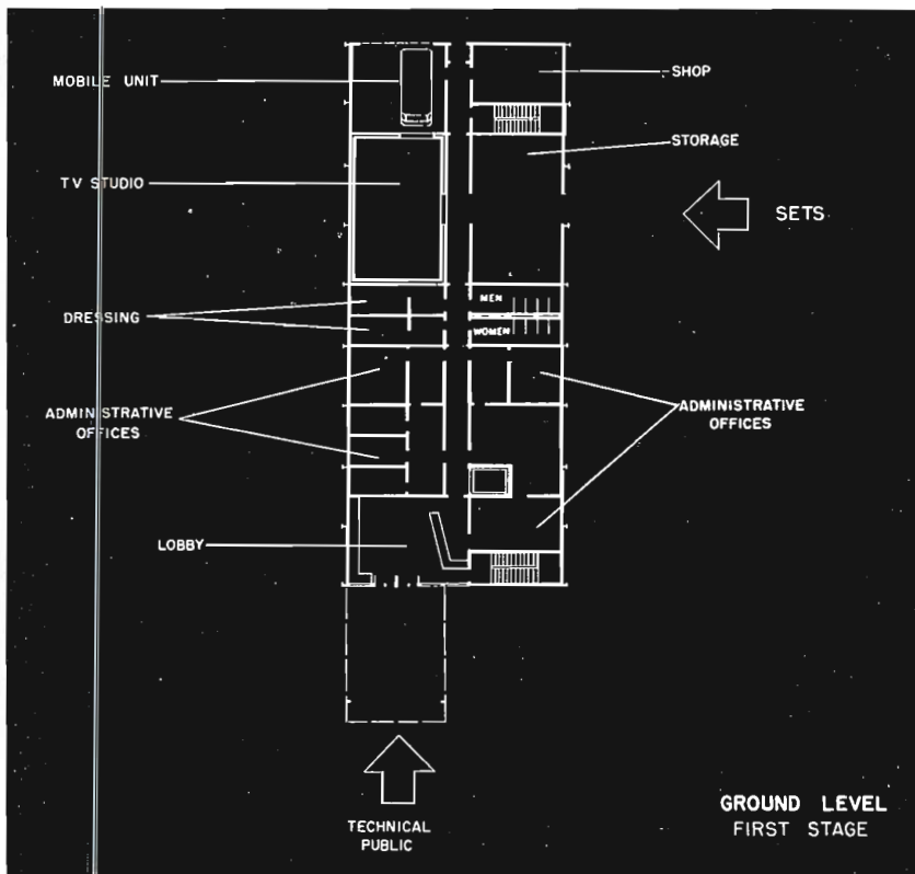
FIG. 8. Plan for ground level, in the first stage.
