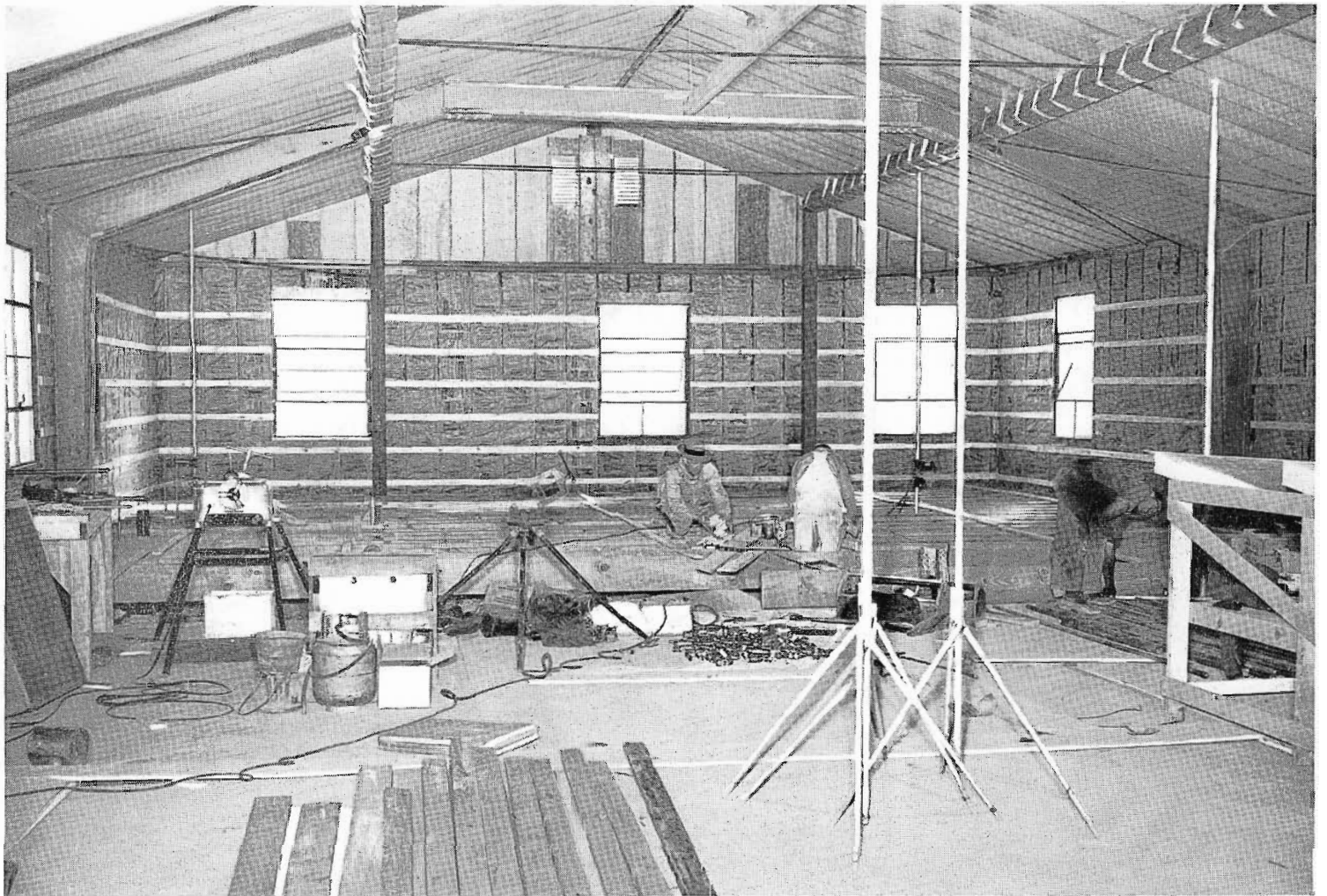
FIG. 5. Interior of the building during construction. All surfaces exposed to outside are covered with 3-incl. fibreglas insulation. The living quarters, which are in the end of the building shown here, have wood floors. The rest of the building has a poured concrete floor.
