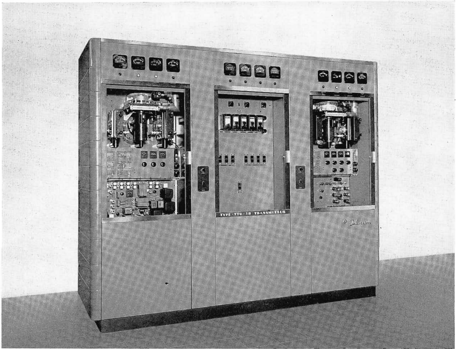
FIG. 2. The TTU-1B may be operated with sliding doors open or closed.
