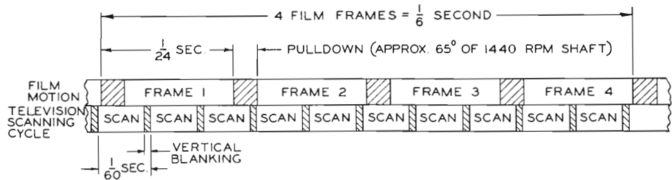
FIG. 5. Time cycling of a standard 16mm projector.
