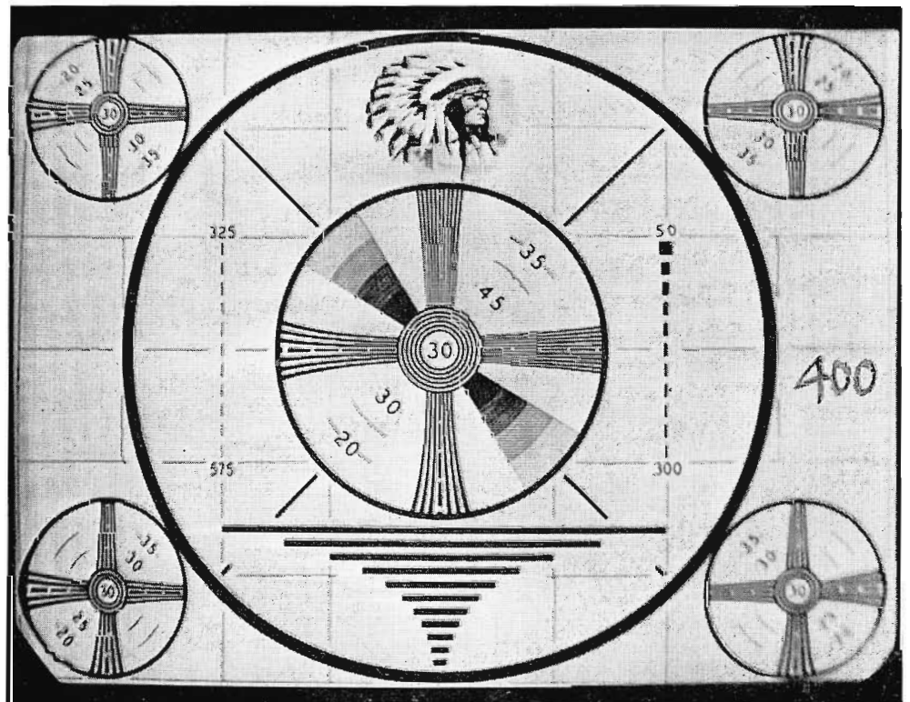
FIG. 16. Kine photo of TTU-1B output.
